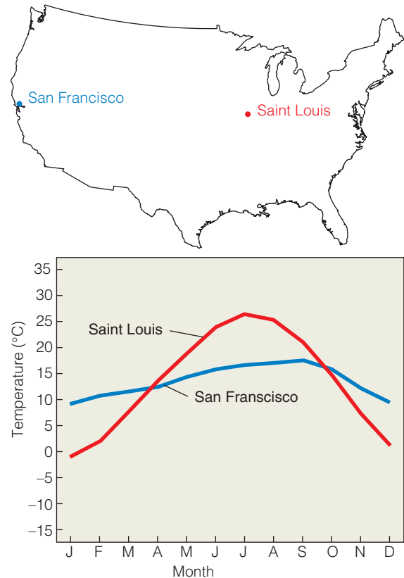
Figure 2.20 Pattern of mean monthly temperature (°C) for two locations in North America: San Francisco is located on the Pacific coast, whereas Saint Louis is in the middle of the continent.
