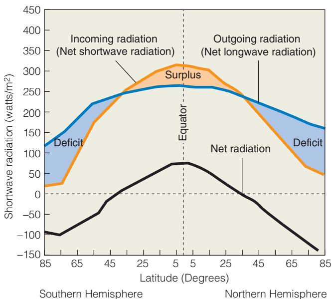
Figure 2.9 Variation in mean annual incoming shortwave radiation, outgoing longwave radiation, and net radiation as a function of latitude. Note that from the equator to approximately 35° N and S latitude, the amount of incoming shortwave radiation exceeds the amount of outgoing longwave radiation, and there is a net surplus of surface radiation (mean annual net radiation > 0). Conversely, there is a deficit (mean net radiation < 0) from 35° N and S to the poles (90° N and S). This gradient of net radiation drives the transport of heat from the tropics to the poles through the circulation of the atmosphere and oceans.
