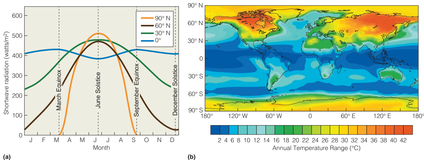
Figure 2.8 Two examples of changes in seasonality with latitude. (a) Annual variations in mean monthly solar (shortwave radiation) for different latitudes in the Northern Hemisphere. (b) Global map of annual temperature range, defined as the difference in temperature (°C) between the coldest and warmest month of the year (based on mean monthly temperatures for the period of 1979–2004).
