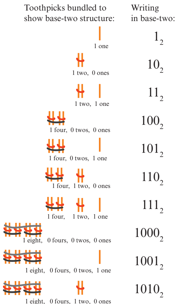
Figure 1.14 The first ten counting numbers in base two.
