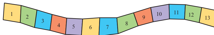
Number paths count “steps.”
